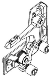
E6940AP1 locks shown (RH c/o)
