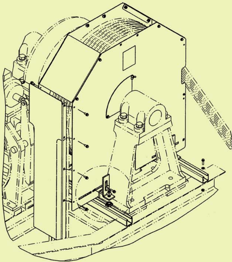
Hollister-Whitney Machine Shown
