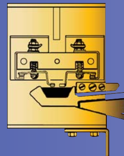
Pre 1962 Switch Contact Assembly
